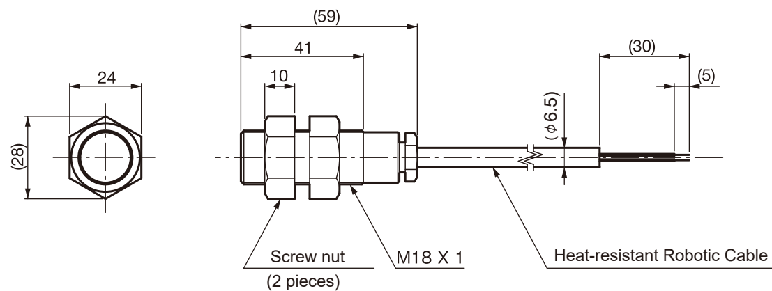
HPS-M18M (Threaded type of sensor)
