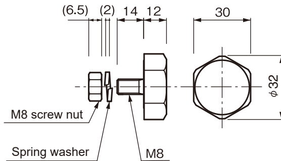
HPM-34 (Magnet)
