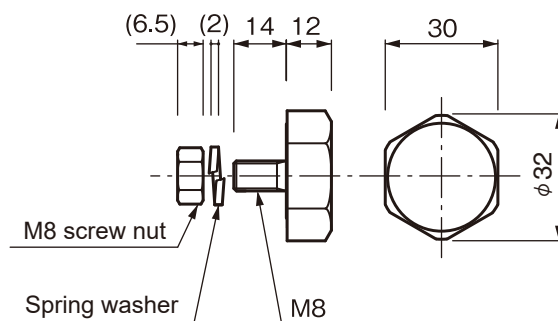
HPM-34 (Magnet)
